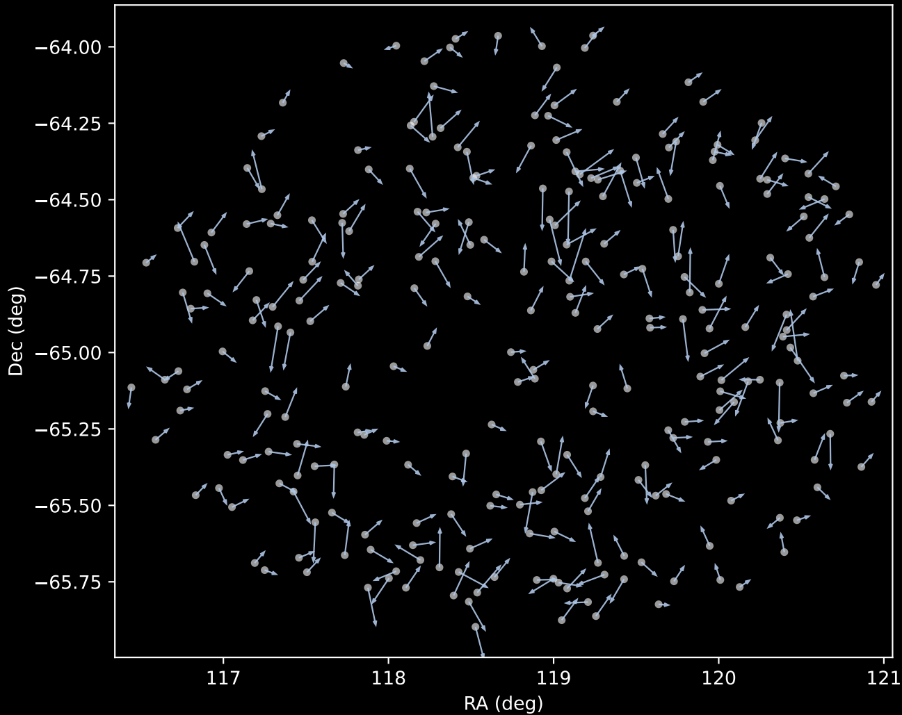
GALAH DR4 Cluster 1 Proper Motion Vectors (n=266)
