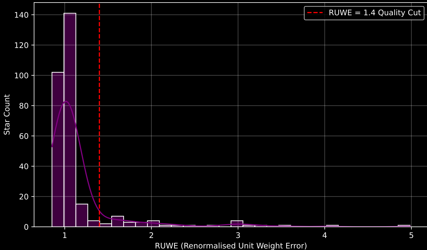
GALAH DR4 Field [6963] RUWE Distribution (n= 294)
