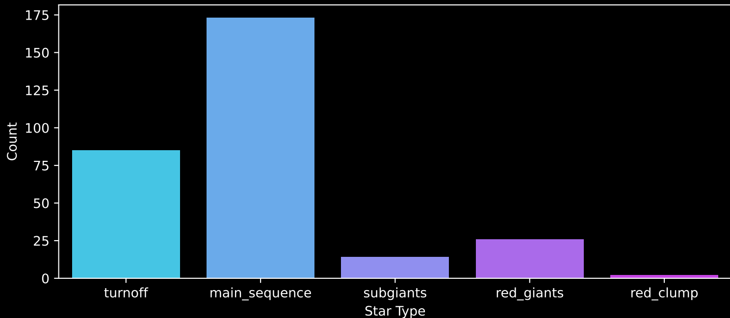
GALAH DR4 Field: [6963] Count plot of Star Type
