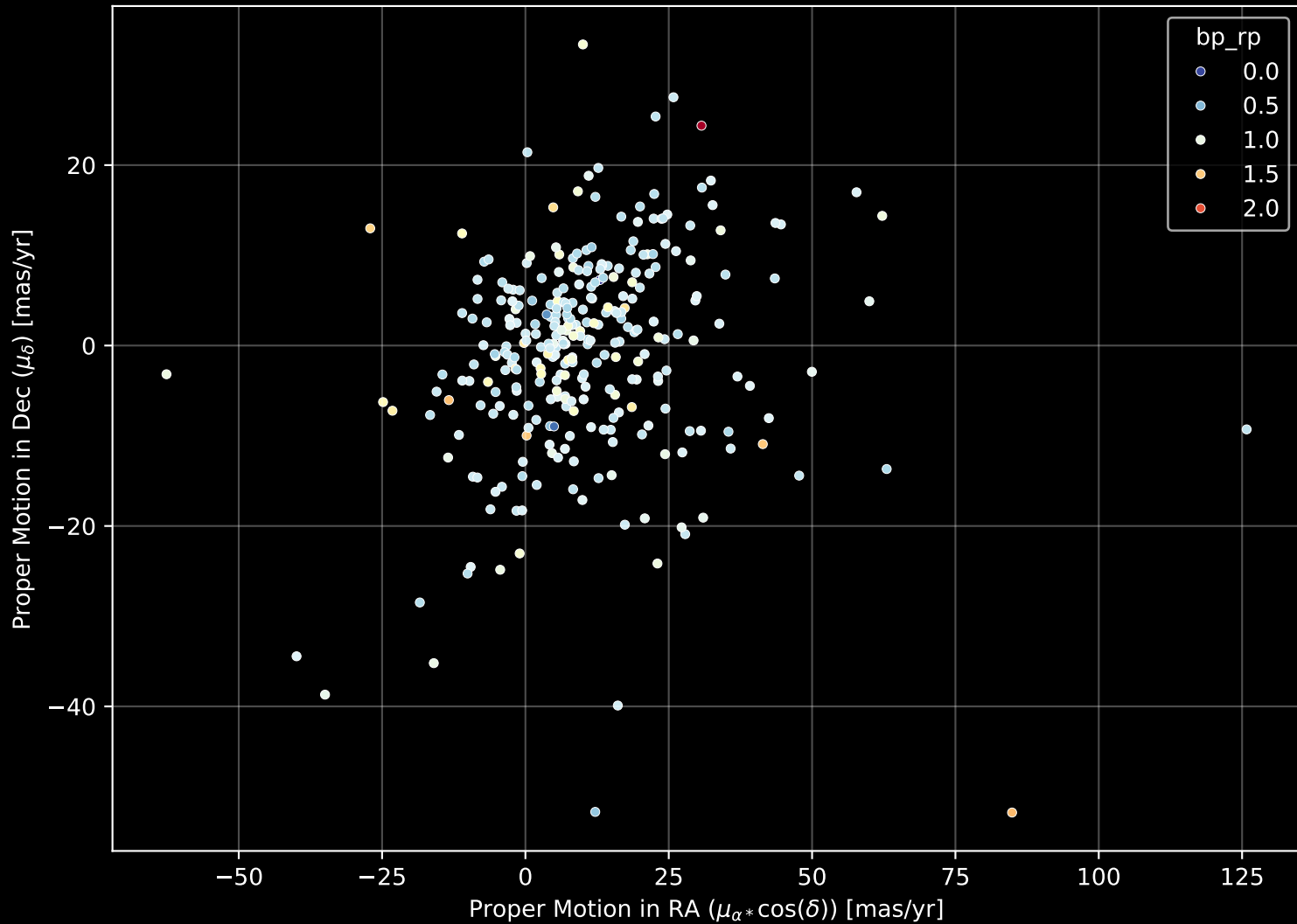
GALAH DR4 Field: [6963] Proper Motion Diagram (n= 300)
